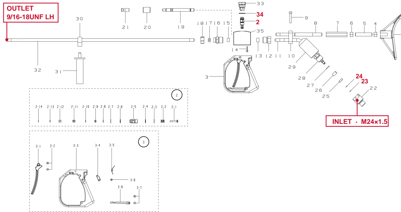
Exploded assembly drawing - callout numbers (incl. sub-assemblies 2-x and 3-x) correspond to the parts list below
